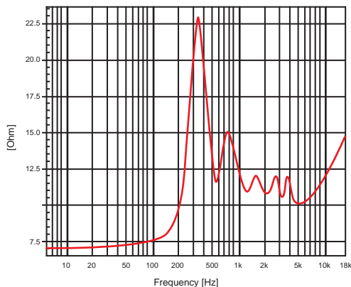
Impedance vs Frequency Response of SSX Be4016 diaphragm measured on a JBL 2446J driver and 2386 horn with a 1.0V rms input.
