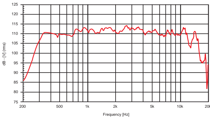
Amplitude vs Frequency of SSX Be4016 diaphragm measured on a JBL 2446J driver and 2386 horn with a 1.0V rms input.
