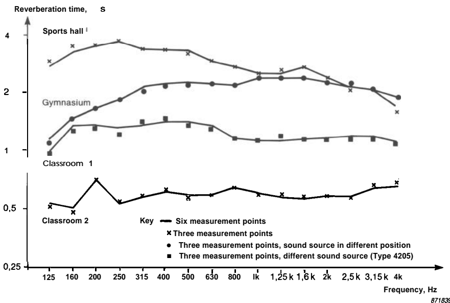
Fig. 3. Spatially averaged T_{(20)} reverberation time results
