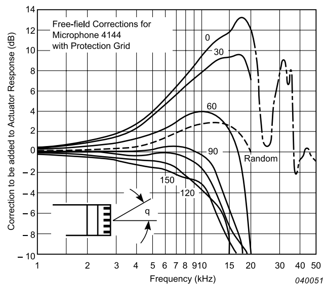
Fig. 1 Free-field correction curves for Type 4144
